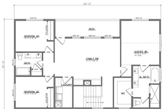
UPPER FLOOR PLAN SCALE: 1/4" = 1'-0"
