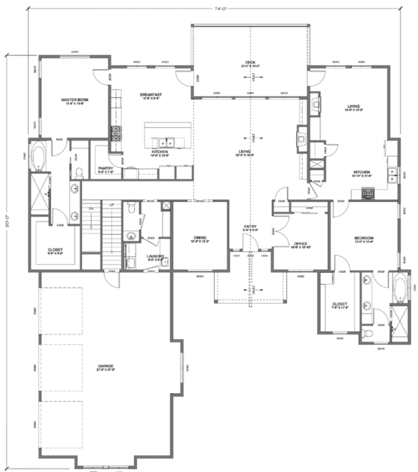
MAIN FLOOR PLAN SCALE 1/4" = 1'
