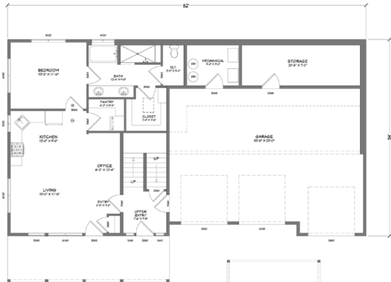
GROUND FLOOR PLAN SCALE 1/4" = 1'
